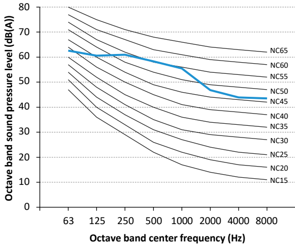
Figure 2-10.4 VMEX010Q8A-D20V335 octave band level
