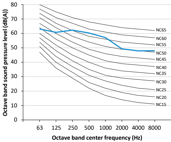
Figure 2-10.6 VMEX014Q8A-D26V450 octave band level
