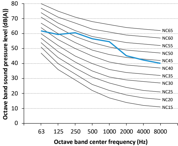
Figure 2-10.3 VMEX009Q8A-D16V280 octave band level
