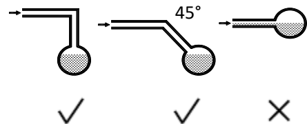
Figure 3-6.3: Branch drain piping joining main drain piping
