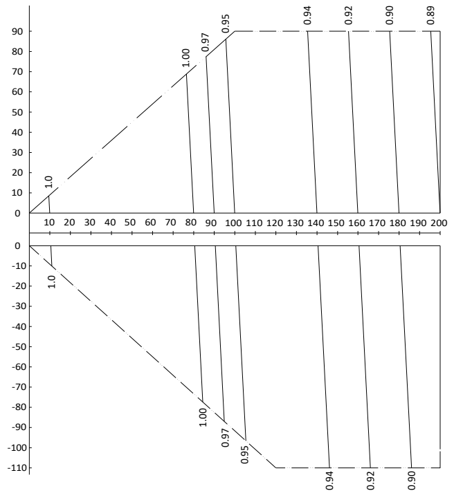
Figure 2-8.6: VMEX018(020)Q8A rate of change in heating capacity
