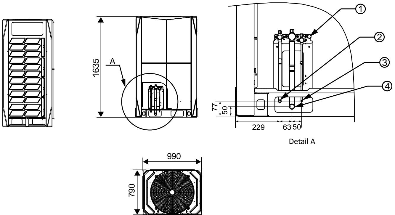
Figure 2-2.1: VMEX008(009,010)Q8A dimensions (unit: mm)
