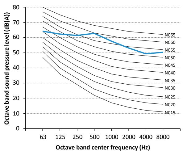
Figure 2-10.9 VMEX020Q8A-D36V615 octave band level
