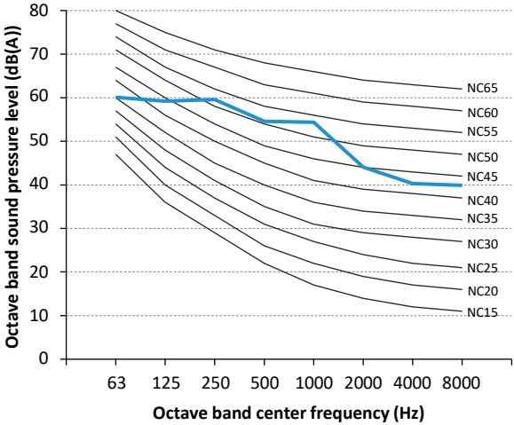
Figure 2-10.2 VMEX008Q8A-D13V224 octave band level
