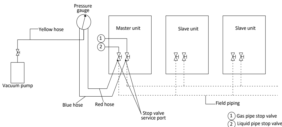
Figure 3-5.14: Vacuum drying
