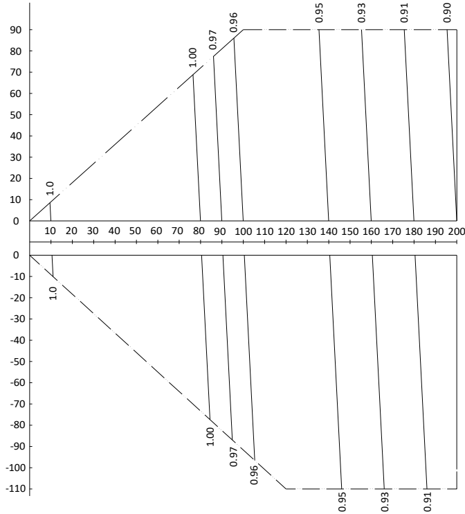
Figure 2-8.4: VMEX012(014,016)Q8A rate of change in heating capacity
