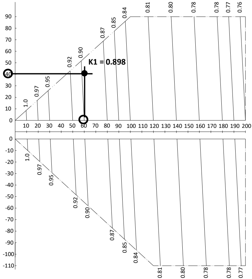
Figure 1-6.3: VMEX018Q8A-D33V560 rate of change in cooling capacity
