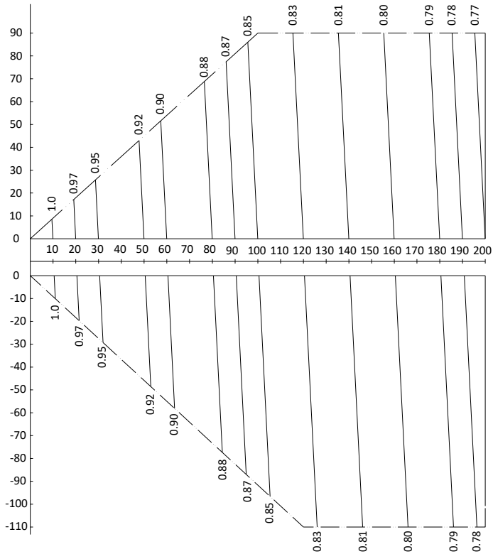
Figure 2-8.3: VMEX012(014,016)Q8A rate of change in cooling capacity
