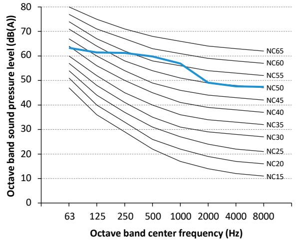
Figure 2-10.5 VMEX012Q8A-D23V400 octave band level
