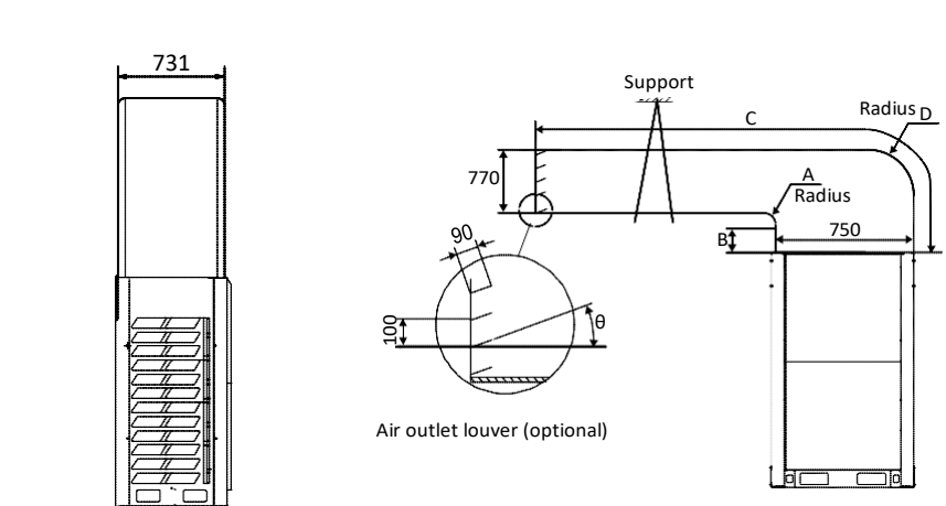
Figure 3-3.3: Longitudinal ducting for VMEX008,009,010 units (unit: mm)
