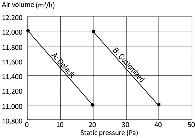
Figure 3-3.6: VMEX008(009) units fan performance
