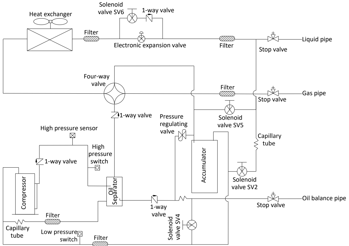
Figure 2-4.1: VMEX008(009,010)Q8A piping diagram
