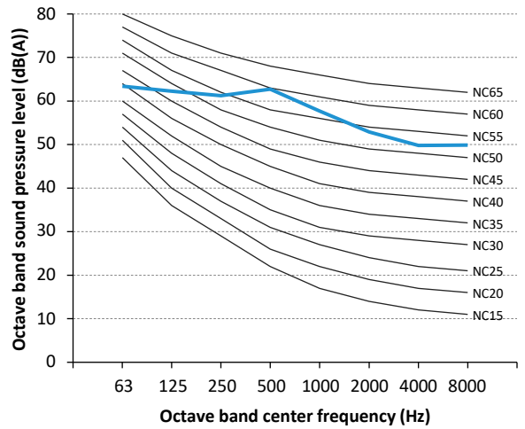
Figure 2-10.7 VMEX016Q8A-D29V500 octave band level
