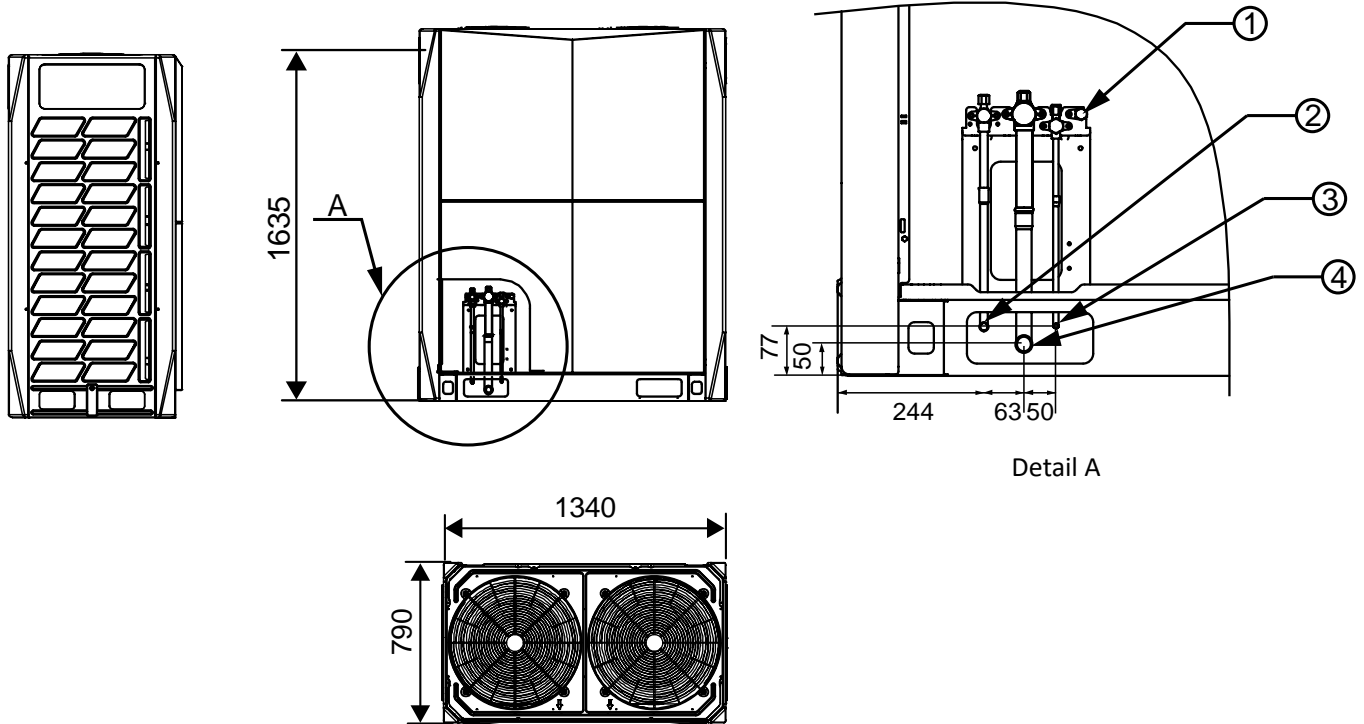
Figure 2-2.2: VMEX012(014,016,018,020)Q8A dimensions (unit: mm)
