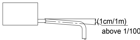
Figure 3-6.1: Drain piping minimum slope requirement
