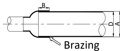
Figure 3-5.7: Piping overlap and gap for brazed joints
