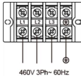
Figure 3-9.3: Outdoor unit 3-phase power supply terminals
