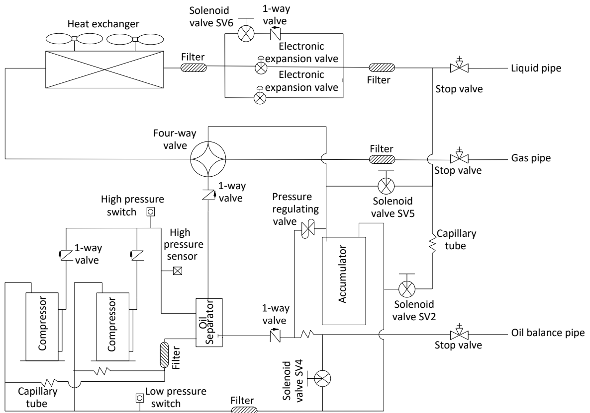
Figure 2-4.2: VMEX012(014,016,018,020)Q8A piping diagram
