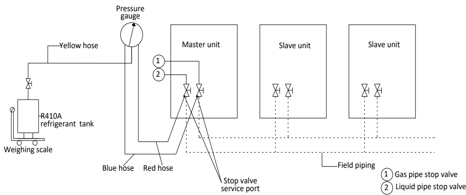
Figure 3-8.1: Charging refrigerant
