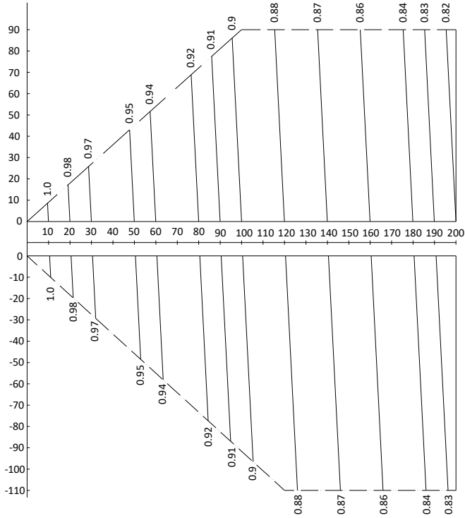
Figure 2-8.1: VMEX008(009,010)Q8A rate of change in cooling capacity
