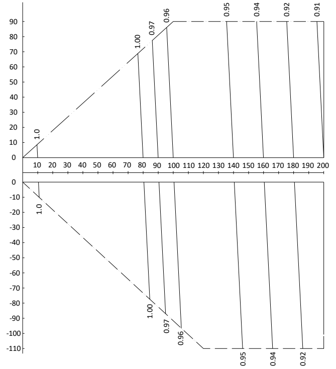
Figure 2-8.2: VMEX008(009,010)Q8A rate of change in heating capacity
