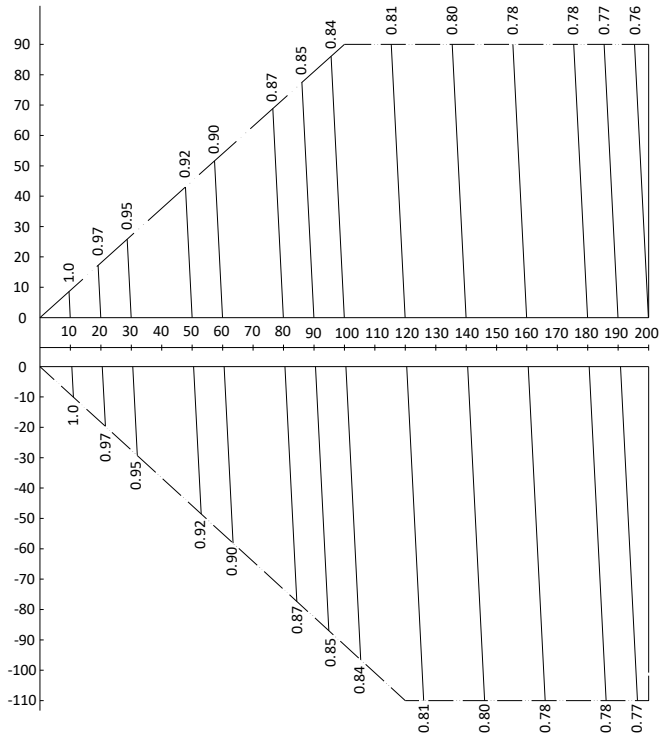
Figure 2-8.5: VMEX018(020)Q8A rate of change in cooling capacity
