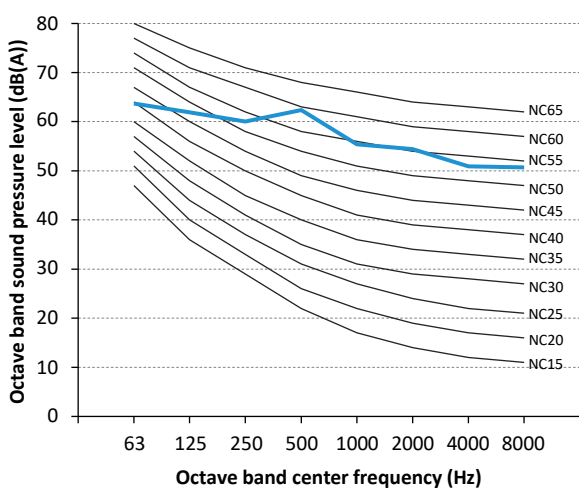
Figure 2-10.8 VMEX018Q8A-D33V560 octave band level
