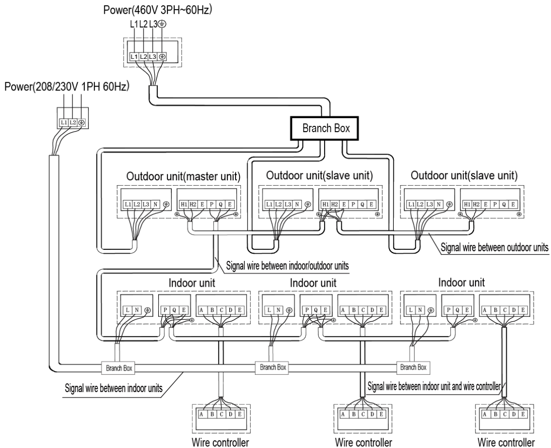
Figure 3-9.6: System power and communication wiring example
