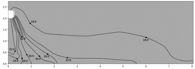
Figure 9.30: VEWM024T0A-DWV071 heating at 300S
