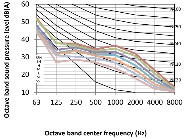
Figure 8.7: VEWM019T0A-DWV056 octave band levels
