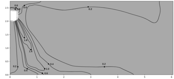
Figure 9.12: VEWM019T0A-DWV056 heating at 300S
