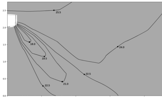
Figure 9.21: VEWM010T0A-DWV028 cooling at 300S
