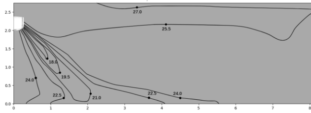
Figure 9.29: VEWM024T0A-DWV071 cooling at 300S
