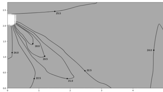
Figure 9.23: VEWM012T0A-DWV036 cooling at 300S
