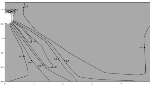
Figure 9.5: VEWM010T0A-DWV028 cooling at 300S
