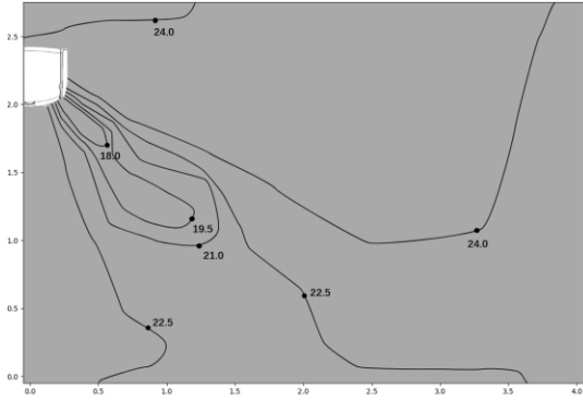
Figure 9.19: VEWM008T0A-DWV022 cooling at 300S
