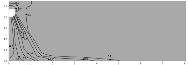
Figure 9.14: VEWM024T0A-DWV071 heating at 300S
