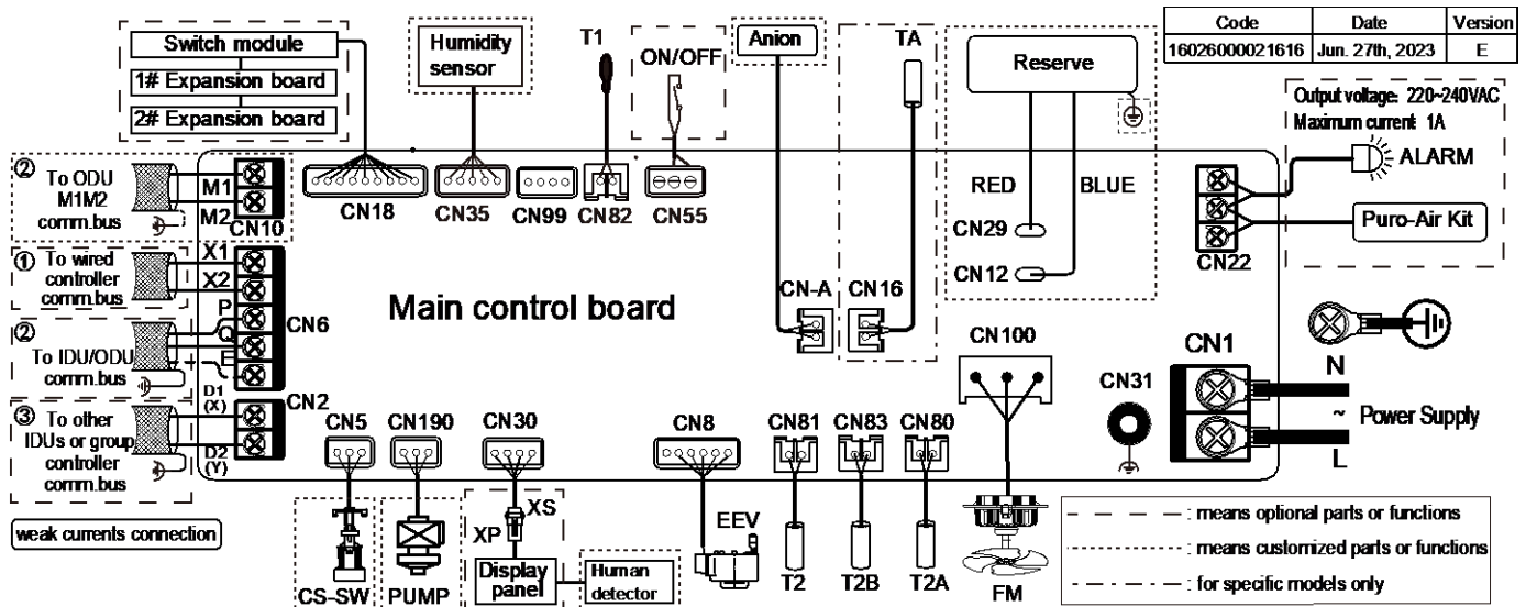
Figure 5.1: VEWM006(008,010,012,015,019,24,27) Wall mounted wiring diagram
