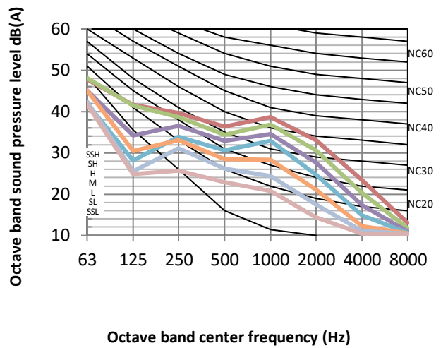
Figure 8.7: VEWM019T0A-DWV056 octave band levels
